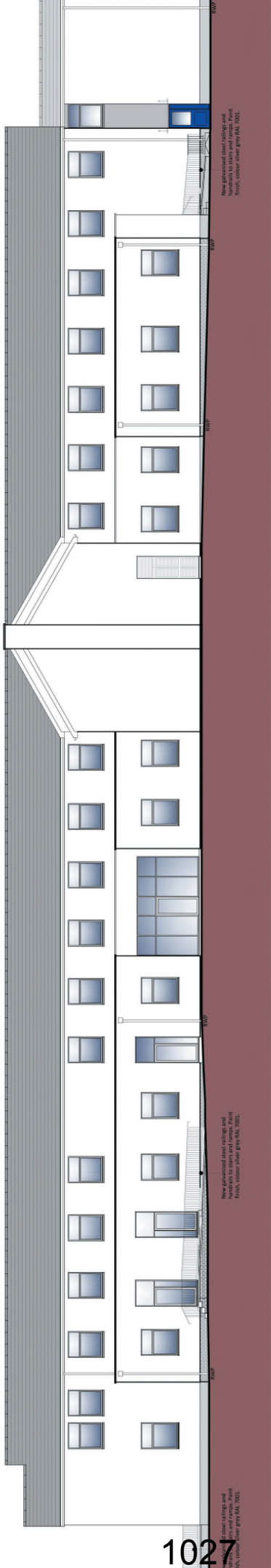
PROPOSED NORTH ELEVATION Scale 1:100@A1
